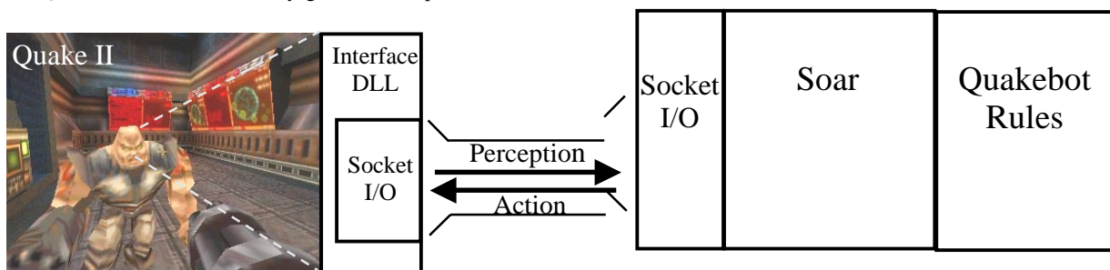
Figure 1. Interface between Quake II and the Soar Quakebot
