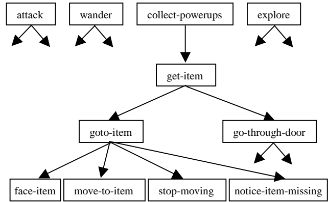
Figure 3. Partial operator hierarchy
